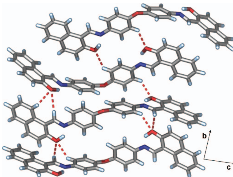
Figure 6. Spatial disposition of the two conformers A and B as viewed along the bc -planes. The two supramolecular dimers of conformer A and B connect via C—H...O and bifurcated C—H...O hydrogen bonds.
